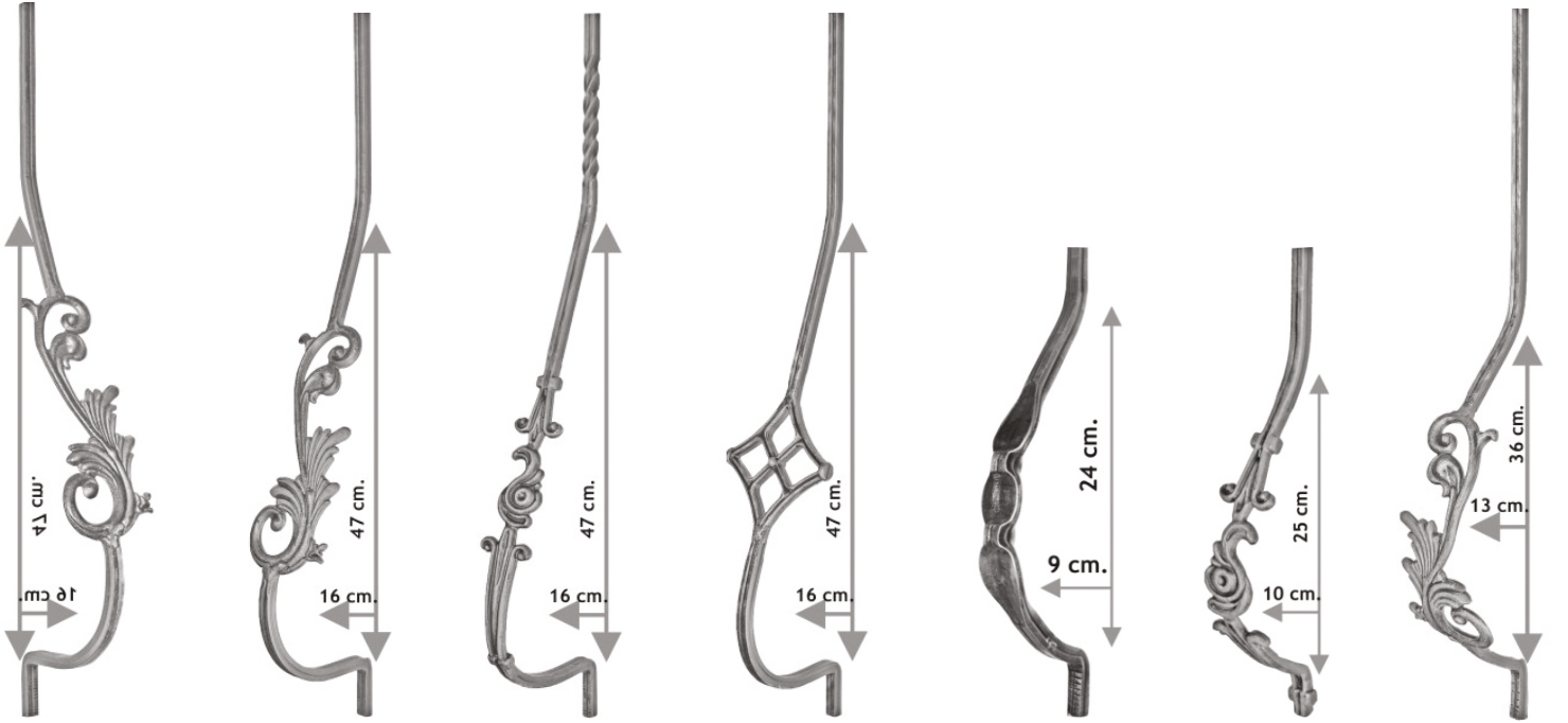
2466-T 600mm-1120gr 800mm-1350gr 1000mm-1580gr ∅12x12
