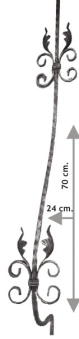
2502 1250mm-2560gr 1500mm-2840gr Ø12x12
